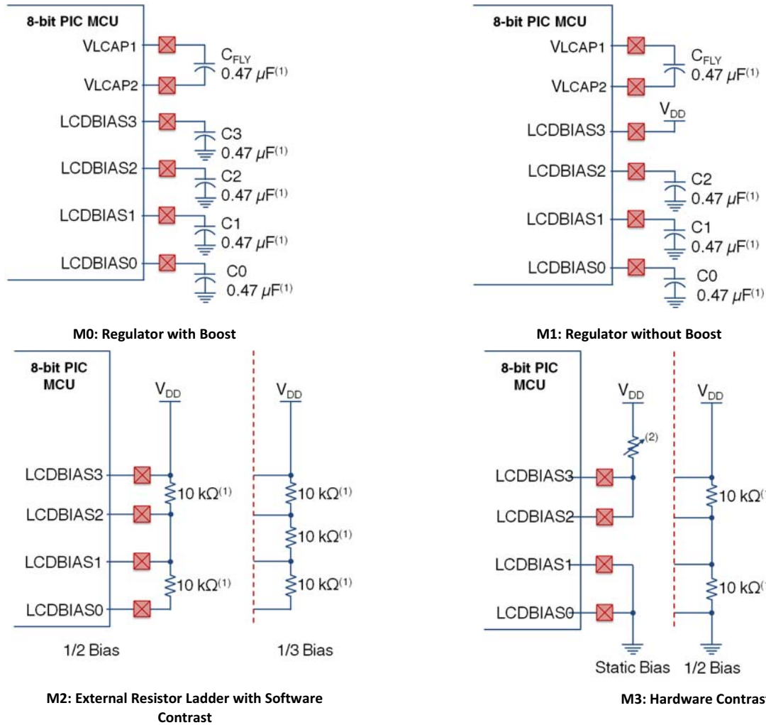
FIGURE 37: LCD BIAS CONFIGURATIONS
