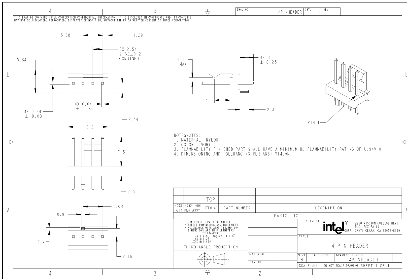
Figure 8 Baseboard Connector
