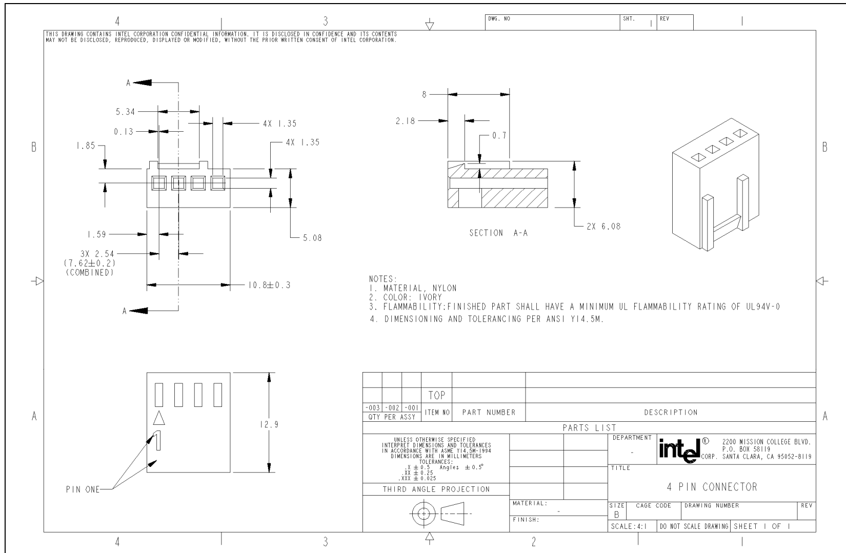
Figure 7 Connector Housing
